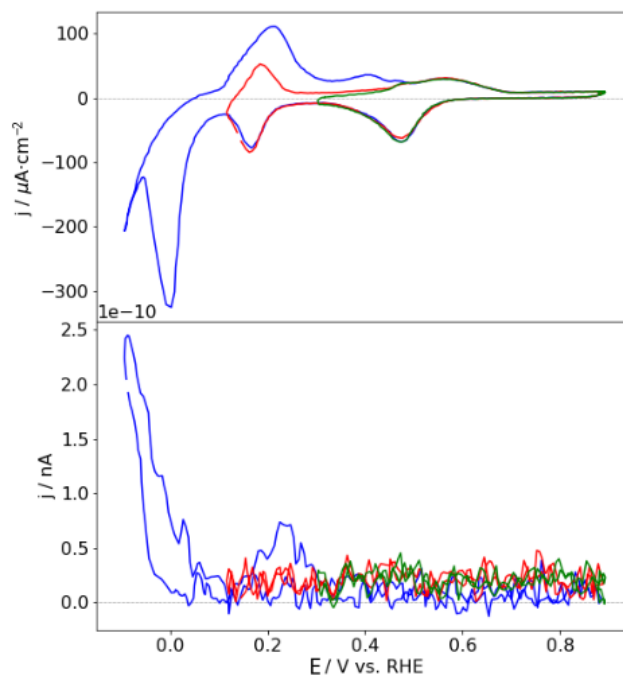
Figure 2: Ru(0001) a) CV b) mass spectrometry recorded with a scanrate of 50 mV/s
